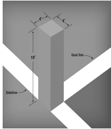
PYLON DETAIL
